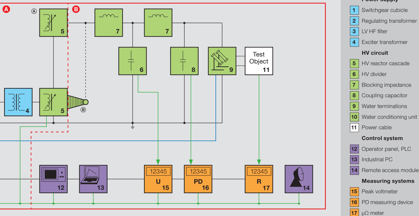
Fig. 2 Principle single-line diagram of cable routine test field
